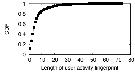
Figure 6: CDF of the length of user activity fingerprints
