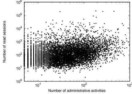
Fig. 8: Total sessions versus number of admin request.
