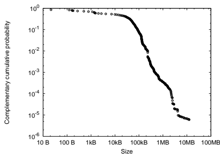
Fig. 1: Marginal distribution (CCDF) of transfer sizes is heavy-tailed, namely a Pareto with parameter \alpha \approx 1 .
