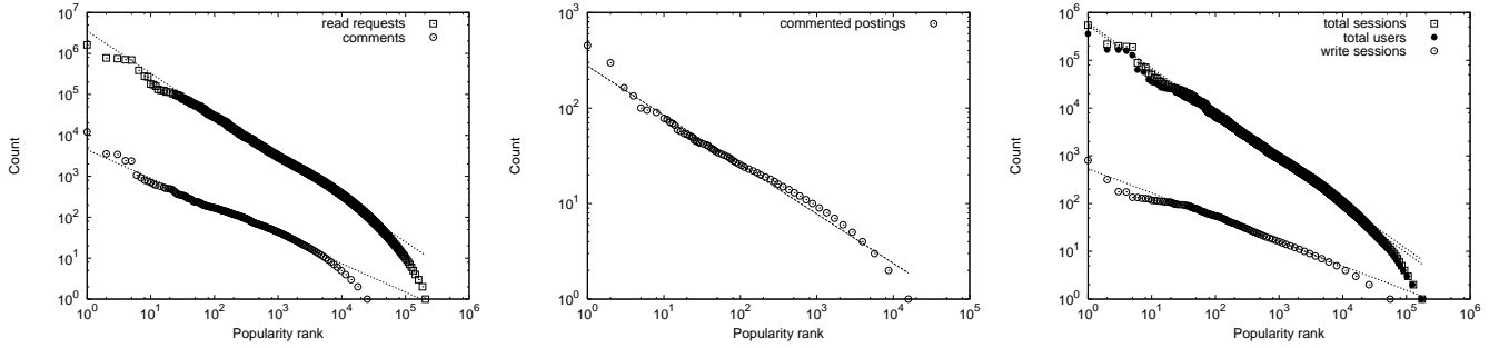
Fig. 7: Popularity profile of blogs: Frequency of read/write requests (left); frequency of commented postings (middle); and frequency of total sessions, write sessions, and users (right) versus rank of blog. All profiles exhibit a power-law relationships.
