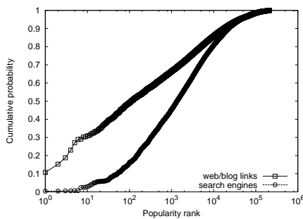
Fig. 5: Cumulative probability that a session will target a blog with a popularity rank smaller than a given value, given that the session's origin is a search engine or a web link.
