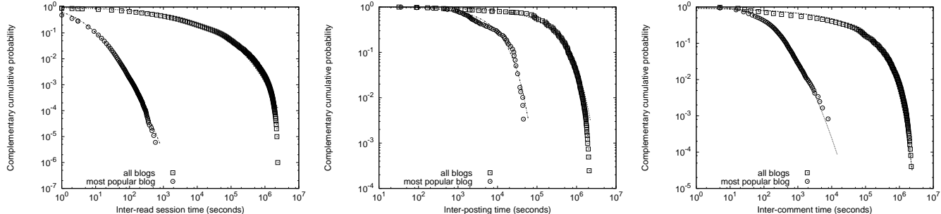
Fig. 10: Distribution of inter-session time (left), inter-posting time (middle), and inter-comment time (right).
